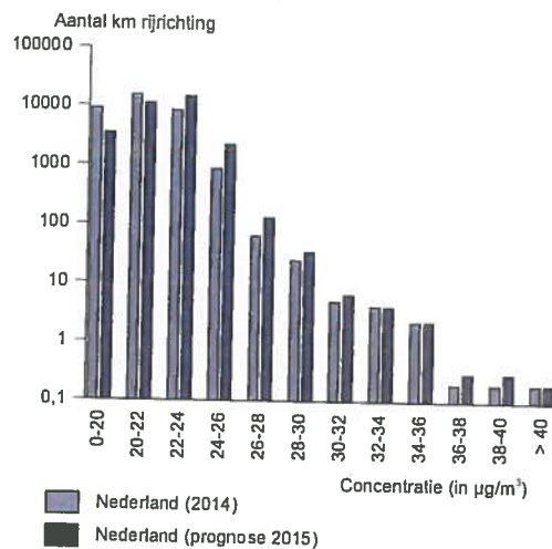
Concentratiehistogram PM_{10}
